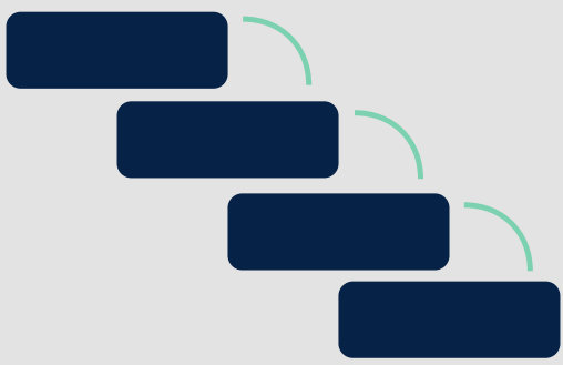
Waterfall validation
