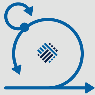
Agile validation
